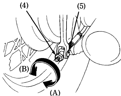
(4) Adjusting nut (5) Arm pin
