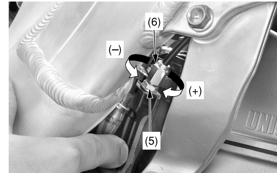
(5) lock nut (6) lower adjuster
