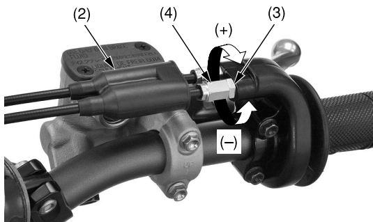
(2) dust cover (3) lock nut (4) upper adjuster
