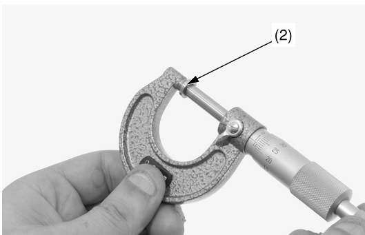
(2) shim
