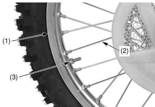
(1) wheel rim (2) spoke (3) rim lock
