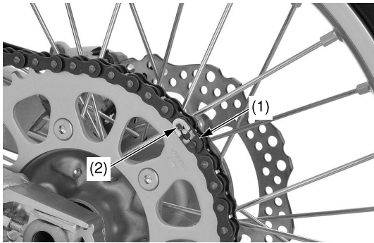
(1) retaining clip (2) master link
