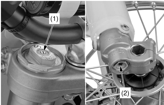
(1) compression damping adjuster (2) rebound damping adjuster
