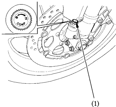
(1) Damping adjuster
