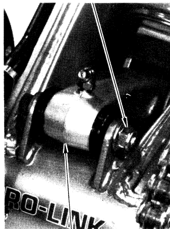
SHOCK ARM
