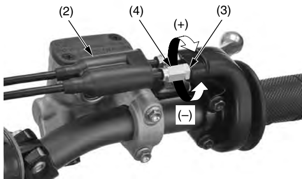
(2) dust cover (3) lock nut (4) upper adjuster (+) increase (-) decrease
