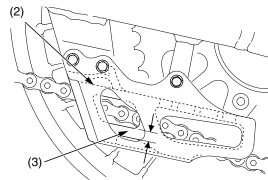
(2) chain guide slider (3) wear indicator
