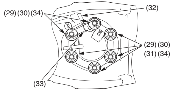
(29) conical spring washers (30) collars (31) washers (32) stopper cable (33) stopper cable guide (34) fuel pump mounting bolts
