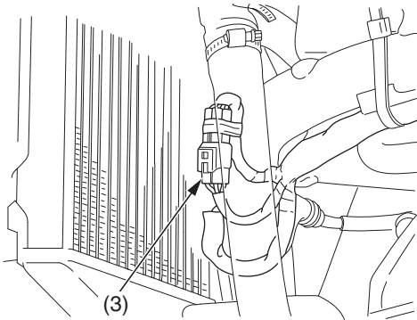
(3) DLC/fuel pump sub harness connector
