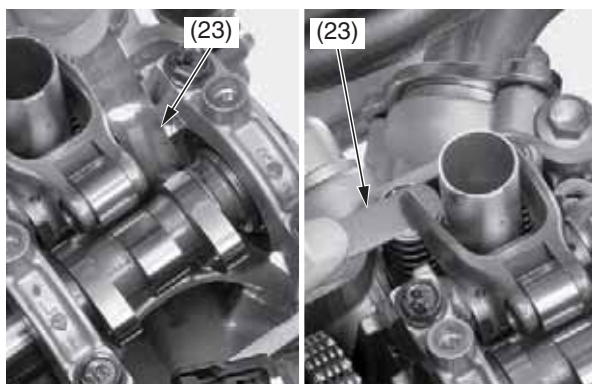
(23) feeler gauge
