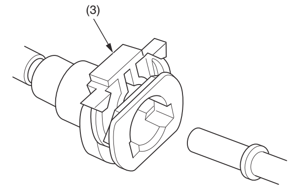
(3) slide retainer
